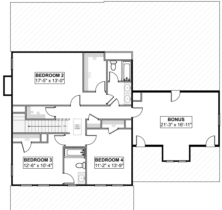
SECOND FLOOR
