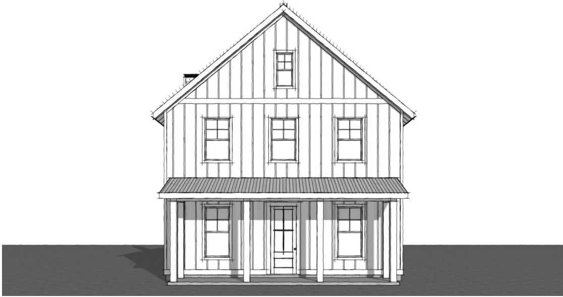
FRONT ELEVATION
