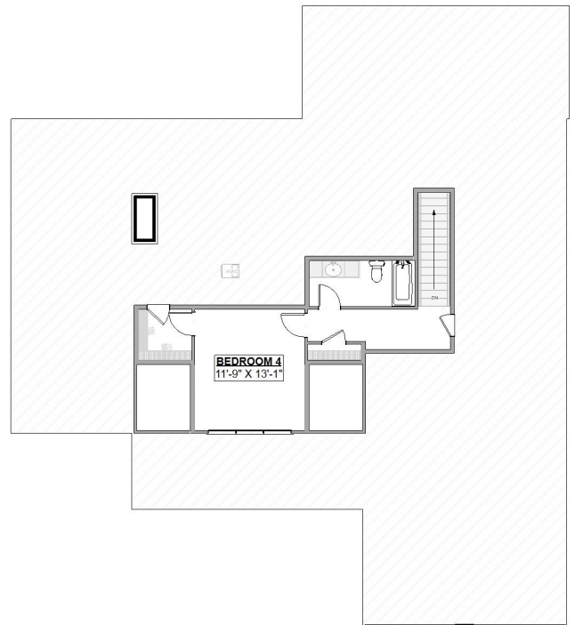
SECOND FLOOR
